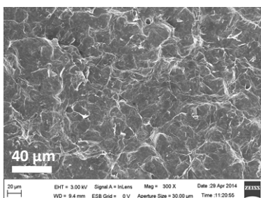
Low magnification scanning electron micrograph showing the morphology of a graphene laminate.
