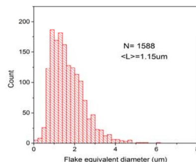
Flake size distribution with an average equivalent diameter of 1.15 µm.
