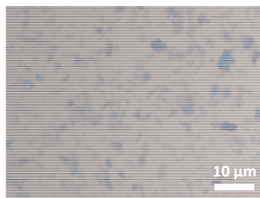
Flakes dropcast from an NMP dispersion on a Si-SiO 2 substrate showing the high yield of monolayer content.
