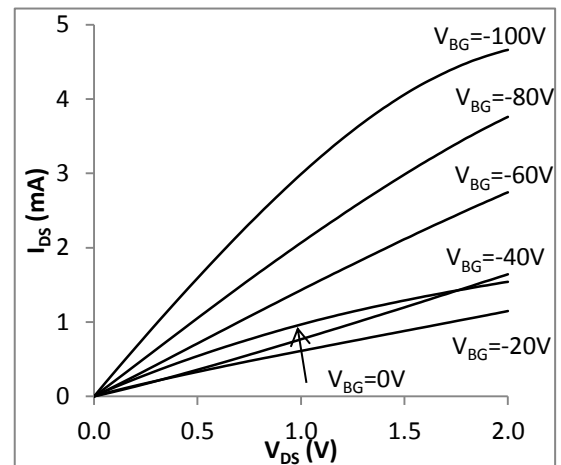
Fig. 2 Drain current vs. drain voltage
